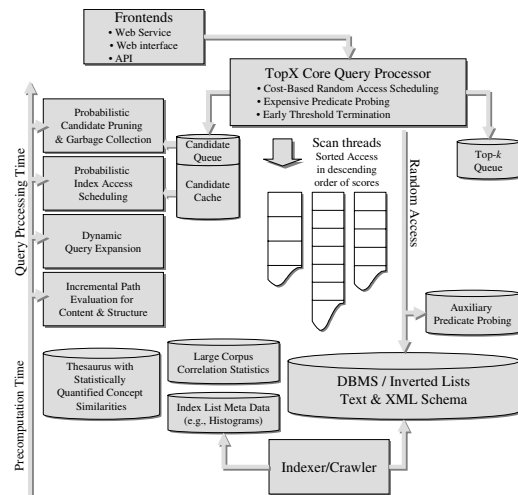
Figure 1: TopX Architecture
