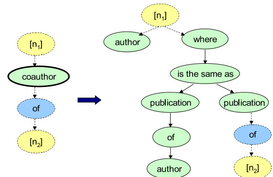
Figure 3: Sample Rule Extracted by DaNaLIX from the iteration in Figure 2(a) (Terms in dashed circles provide context for rule-based transformation only.)
