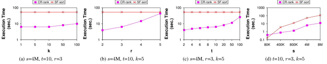
Figure 8: Ranking Efficiency.
