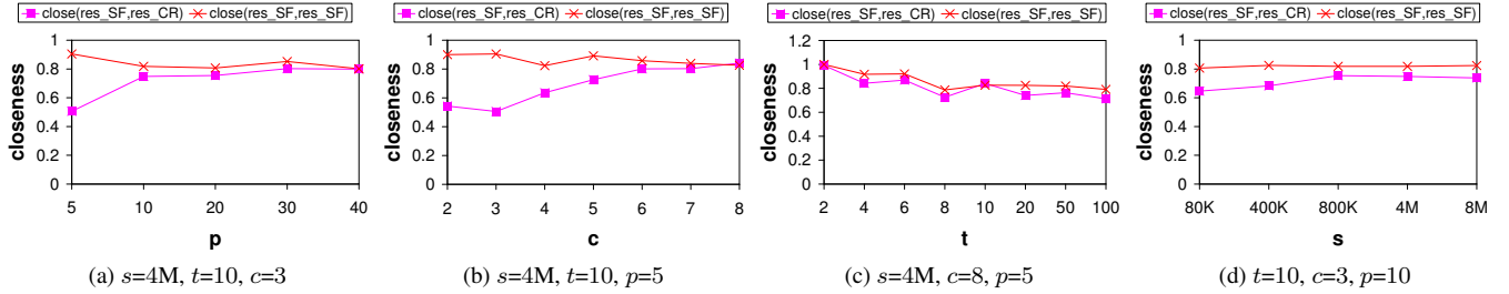
Figure 7: Clustering Quality.
