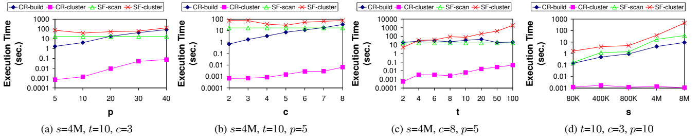
Figure 5: Clustering Efficiency.
