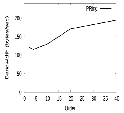
Figure 14. Bandwidth Cost
