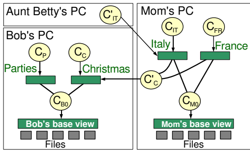
Figure 5: Solving the photo sharing scenario with views and capabilities. Rectangles denote views, e.g. , ‘Christmas’ is the view of all Bob’s Christmas photos; circles denote capabilities, e.g. , C_C is Bob’s capability to his ‘Christmas’ view. C'_C is a copy of C_C that Bob sent to Mom to share the ‘Christmas’ view with her. Mom’s ‘Italy’ view composes two capabilities, C'_C and C_{M0} .
