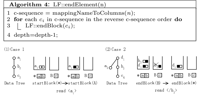
Figure 6: LF: Incorrect order of calling blocks (query: '//*[//A]/B/C' ).
