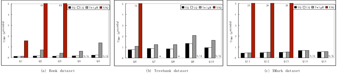
Figure 14: Query time 7 .
