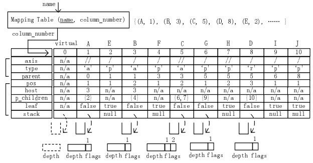
Figure 3: Query table for the query of Figure 2.
