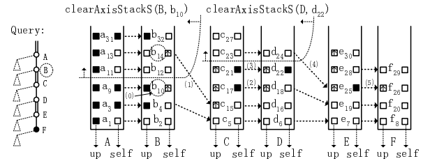
Figure 10: U-EQ: top_down_Propagate( b_{10}b_{14} ) .
