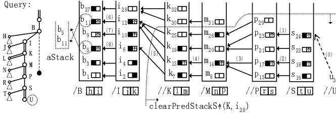
Figure 9: U-EQ: bottom_up_Evaluate(U) .
