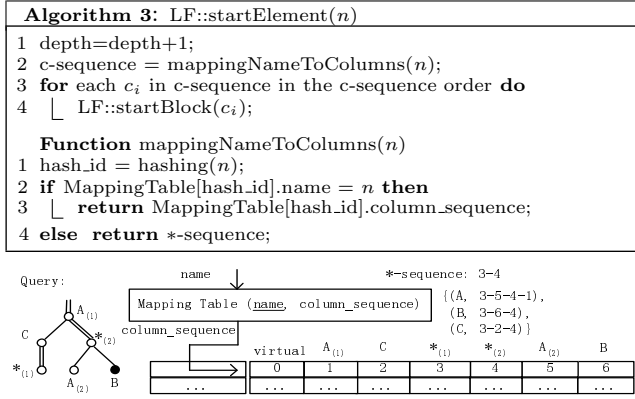
Figure 5: Mapping table (LF): name \rightarrow column sequence.
