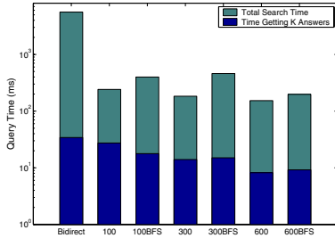
Figure 9: Performance on IMDB
