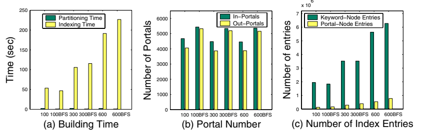
Figure 10: Impact on indexing the IMDB graph with various parameters.
