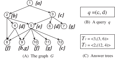
Figure 1: Example of query and answers.
