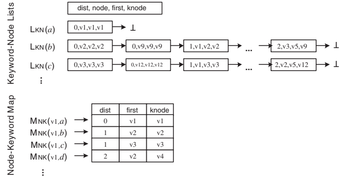
Figure 4: Keyword-node lists and node-keyword map.
