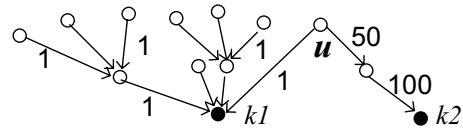
Figure 3: An example where distance-balanced expansion across clusters performs poorly.
