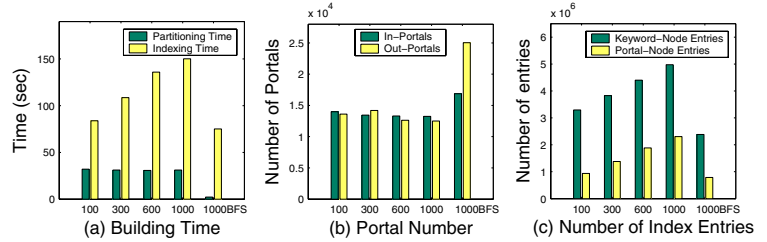
Figure 8: Impact on indexing the DBLP graph with various parameters.
