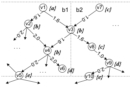
Figure 5: Example of portals and blocks.
