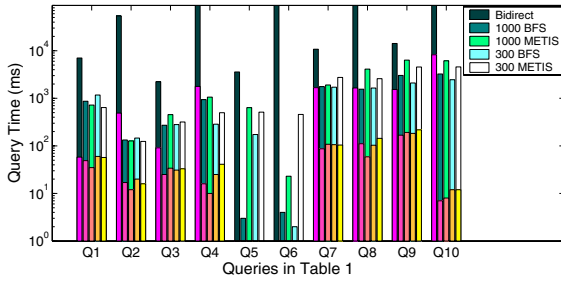
Figure 7: Query performance on the DBLP graph.
