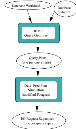
Figure 5: Generating I/O Request Sequences
