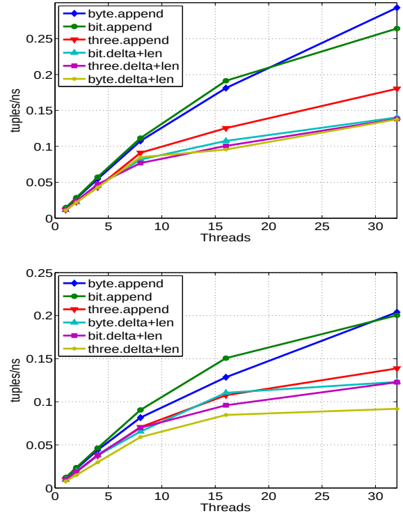
Figure 6: Scan Bandwidth on the Sun-T1 for a scan (Q1b:top) and a predicate on a variable length field (Q3:bottom)
