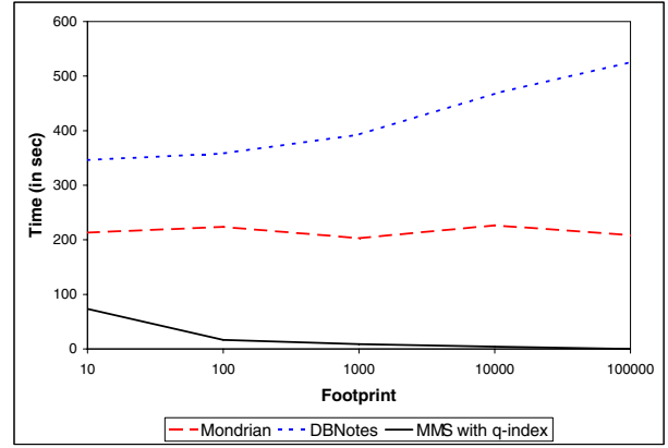
Figure 7: Average query execution time.
