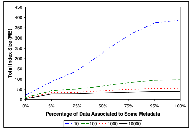
Figure 6: Q-Index size for different footprints.
