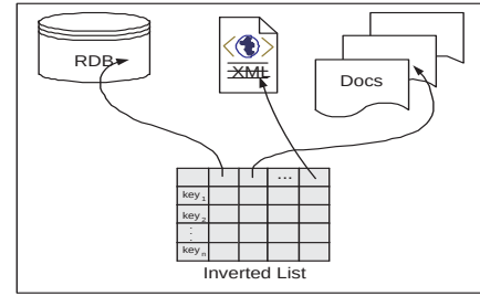
Figure 1: We build an index over a collection of heterogeneous data. Our index is an inverted list where each row represents a keyword and each column represents a data item from the data sources.
