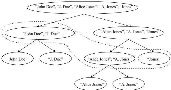
Figure 5: Search Space of Partitions
