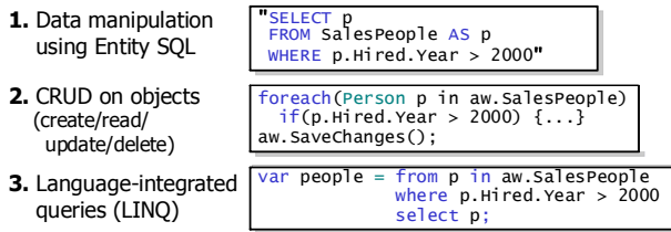
Figure 1: Interacting with data in the Entity Framework
