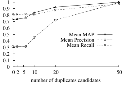
Figure 7: Sensitivity to Pre-selected Duplicates
