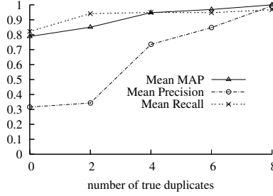
Figure 8: Sensitivity to True Duplicates
