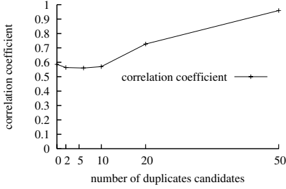
Figure 10: Accuracy in Correlation Quantification
