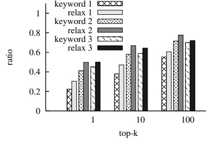
Figure 11: Chance of Finding Intended Item in Top-k Results
