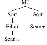
Figure 7: SMJ S plan.
