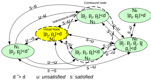
Figure 5: Index for Conflicting and Harmonious Constraints
