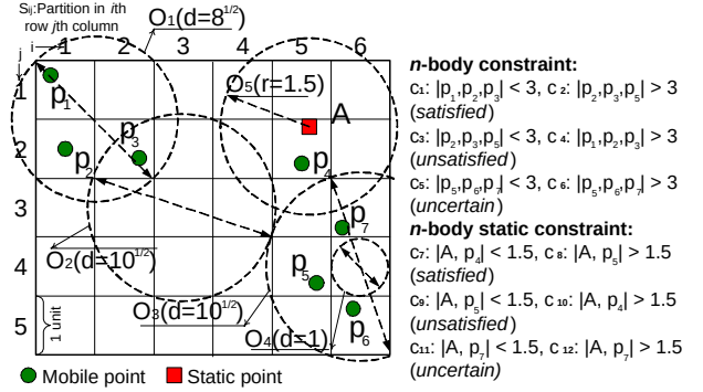
Figure 2: Illustration of Partition-based Evaluation
