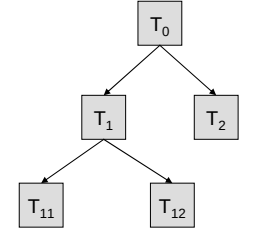
Tree-structured Schema
