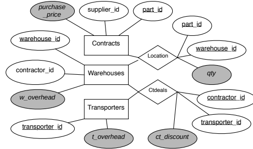
Figure 1: A supply chain decision support schema. Measure attributes are shaded.
