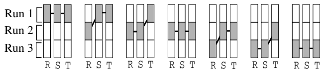
Figure 4: Using the round-robin method, seven combinations of runs are considered when relations R , S , and T (each broken into three runs) are sorted during the scan phase of a levelwise step.
