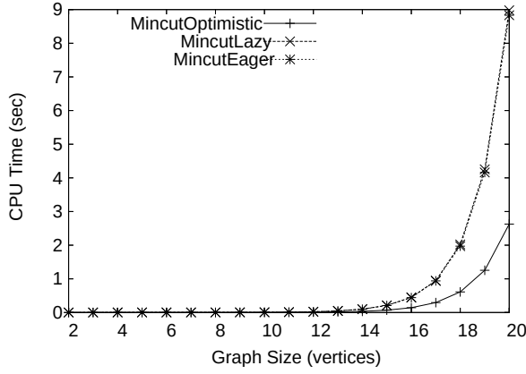
Figure 4: Minimal Cuts of Clique Graphs
