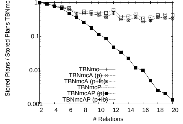
Figure 8: Storage Size: Star Queries, Bushy
