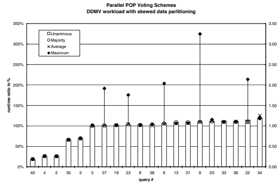
Figure 9: Runtime ratio of DDMV queries using different voting schemes.
