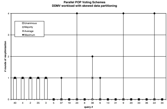
Figure 8: Number of re-optimization rounds for DDMV queries using different voting schemes.
