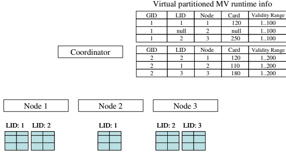
Figure 3: Example of intermediate results reuse based on VPMVs.
