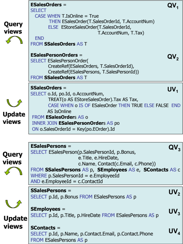
Figure 6: Bidirectional views for mappings in Figure 5
