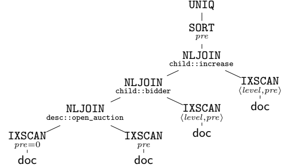
Figure 3: DB2 execution plan corresponding to the path /descendant::open_auction/bidder/increase .
