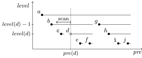
Figure 7: XPath parent navigation by means of a reverse \langle \text{level}, \text{pre} \rangle index scan (starting from context node d ).
