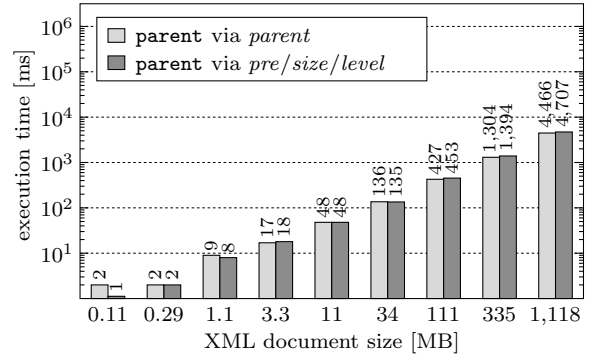
Figure 9: The evaluation of parent using a partitioned \langle \text{level}, \text{pre} \rangle index is almost on par with the foreign key-based alternative (path /\text{descendant}::\text{description}[\text{parent}::\text{node}()] ).
