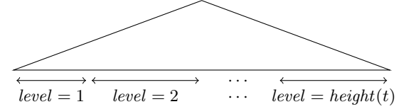
Figure 4: B-tree partitioning.
