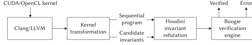
Fig. 1. The GPUVerify architecture, which draws on the Clang/LLVM and Boogie frameworks
