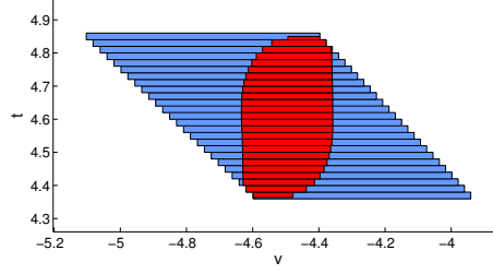
This figure shows the first intersection of a bouncing ball with the guard (the floor). For the model description see Sect. 5. We used the time step \delta = 0.02 . The outer slices show the intersections computed by Algorithm 2 using a rectangular template matrix. Each inner slice shows a tight rectangular over-approximation of the sops computed by Algorithm 1. Their
