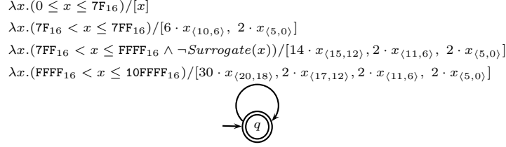
Fig. 1. SFT EncUTF8 : UTF8 encoder for valid Unicode code points; x_{\langle h,l \rangle} extracts bits from h to l from x , e.g., 8_{\langle 3,2 \rangle} = 2 ; \text{Surrogate} \stackrel{\text{def}}{=} \lambda x. D800_{16} \leq x \leq DFFF_{16} , surrogates are not valid code points; x \cdot y denotes bit-append, e.g., 6 \cdot x_{\langle 10,6 \rangle} = C0_{16} + x_{\langle 10,6 \rangle} .
