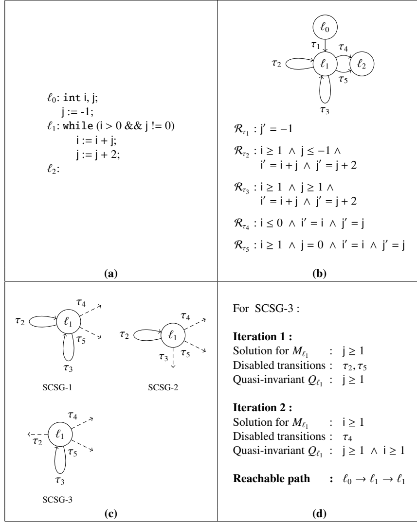
Fig. 1. Example program (a) together with its corresponding CFG (b), non-trivial SCSGs (c) and non-termination analysis (d)
