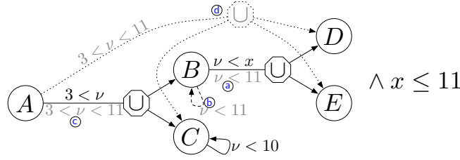
Fig. 1. Example QUIC graph and accompanying numeric domain instances, showing a sequence of inferences: \textcircled{a} is derived by pushing the external numeric domain fact x \leq 11 and \nu < x ; \textcircled{b} is derived by inferring a new self-loop with \top and pushing \textcircled{a} ; \textcircled{c} is derived by pushing \textcircled{b} \sqcup \nu < 10 and 3 < \nu ; and \textcircled{d} is derived by inference/transitive closure of the graph.
