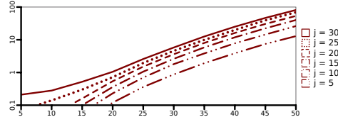
Fig. 3: JUDGEHASH's running times in seconds (ordinate) in terms of the word length i (abscissa) for G_{\text{art},i,j} vs. G'_{\text{art},i,j} .
