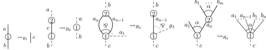
Fig. 2. structurals ( R_1, R_2 ), multiplicative ( R_3 ) and associative ( R_4 ) retractions
