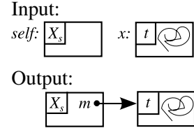
Figure 7: Graph fragments for input and output of the function type in the example.
