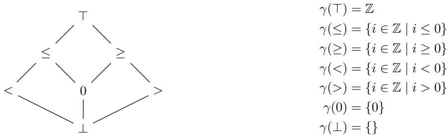
Figure 1: Abstract domain lattice for sign analysis
