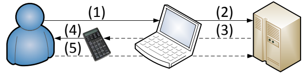
Fig. 1. The transaction information flow in CVTSA methods. A secure device, provided by the bank, is used to present transaction requests received by the bank to the customer for authentication. Dashed lines represent information flows which are optionally forwarded by the traversed devices, depending on the type of authentication device.
