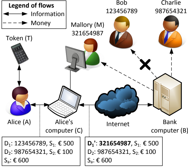
Fig. 3. Alice fails to transfer money to Bob.
