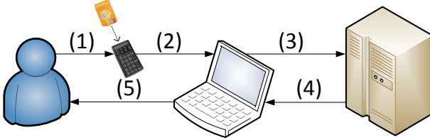
Fig. 2. The transaction information flow of our proposed WYEWYS-based authentication method for single transaction requests.
