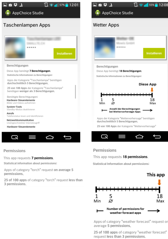
Fig. 2. Original “Text UI” (upper left), original “Graphic UI” (upper right), translation of “Text UI” (lower left), and translation of “Graphic UI” (lower right).
