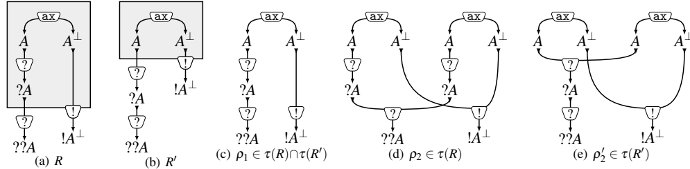
Figure 1: Two different proof-nets R (Fig. 1(a)) and R' (Fig. 1(b)), having the same 1-diffnet \rho_1 (Fig. 1(c)) but two different 2-diffnets, \rho_2 (Fig. 1(d)) and \rho_2' (Fig. 1(e)) respectively.
