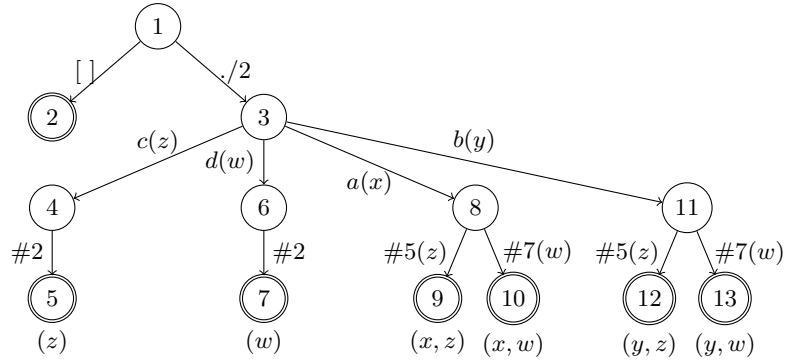
Fig. 2. Index for example terms ( rtype lst \rightarrow [] ; [nv|lst]:::index([0,1,2]) )
