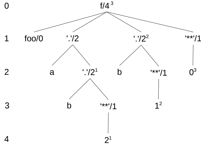
Fig. 1. Rational term: f(foo, [a,b|cycle_at_depth(2)], [b|cycle_at_depth(1)], cycle_at_depth(0)) in tree notation
