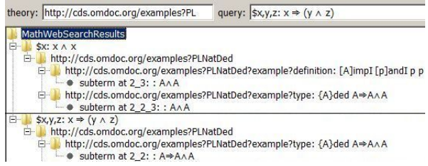
Figure 7: Display of Search Results
