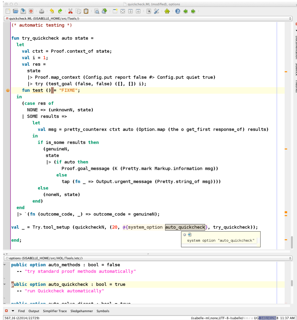
Figure 4: Live editing and browsing of Isabelle/HOL ML files
