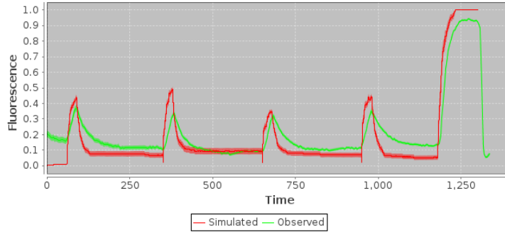
Fig. 5: Simulated fluorescence traces for inferred parameters
