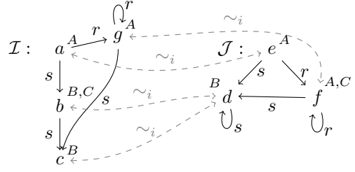
Figure 4: Computation of (\mathcal{I}, a) \sim_i (\mathcal{J}, e) by pairing their successors and recursively computing \sim_i between those.
