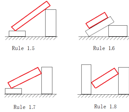
Figure 6: ERA-stable cases of angular rectangles
