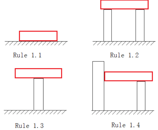
Figure 5: Examples for ERA-stable cases of regular rectangles
