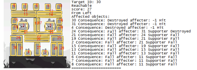
Figure 11: Level 1-16 in Chrome Angry Birds and agent output for this level
