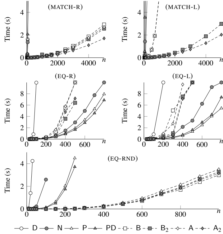
Fig. 6: Evaluation results
