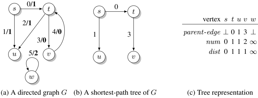
Fig. 1: A directed graph G = (V, E) with the edges labeled i/k , where i is a unique edge index and k is the cost of that edge is presented in (a). In (b) we give a shortest-path tree of G that is rooted at start vertex s \in V . The tree is encoded by parent-edge , num , and dist according to the table in (c). Observe that vertex w is not reachable from s and that the cycle t \rightarrow v \rightarrow t has cost zero.
