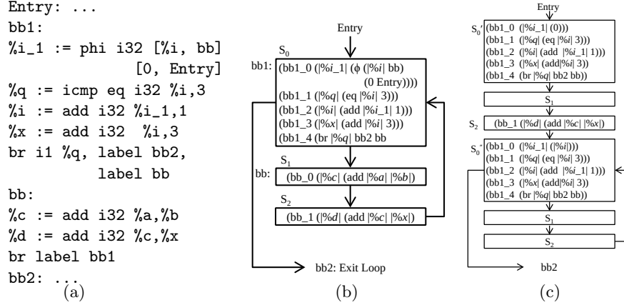
Fig. 1. (a) Loop in LLVM Assembly (b) Fragment of CCDFG corresponding to loop. Scheduling step S_0 has a \phi -statement (c) \phi -elimination operation. \%i_1 is assigned 0 in S'_0 and \%i in S'_1 .
