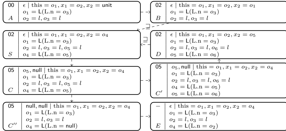
■ Figure 2 The (incomplete) computation graph of append .
