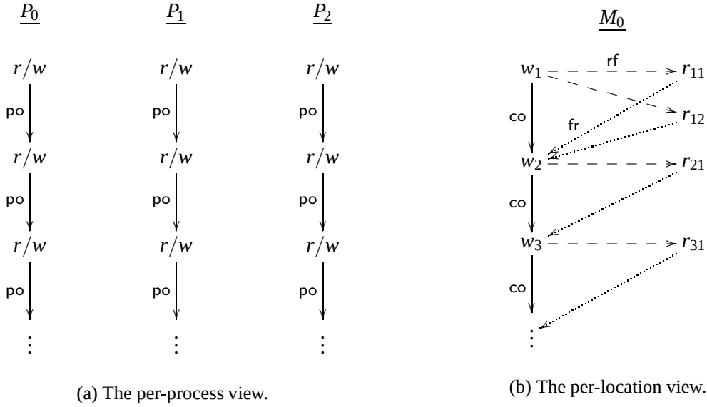
Figure 2: Two views of memory events. In figure (b), solid lines are co , dashed lines are rf , and dotted lines are fr . For po , co and fr , not all arrows are pictured, as po and co are transitively closed.
