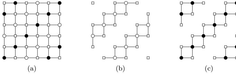
Fig. 2: Incidence graph of a QDNF formula (a). Universal variables are drawn with black round shapes, existential variables with white round shapes, and terms are drawn with square shapes. Both deleting the universal variables (b) and the existential variables (c) significantly decreases the treewidth of the incidence graph.
