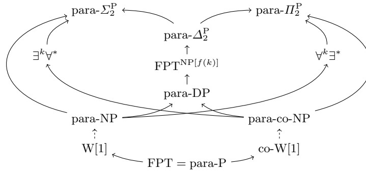
Fig. 1: Parameterized complexity classes up to the second level of the polynomial hierarchy. Arrows indicate inclusion relations. (We omit the full definition of some of the parameterized complexity classes depicted in the figure. For a detailed definition of these, we refer to other sources [13,17,35].)
