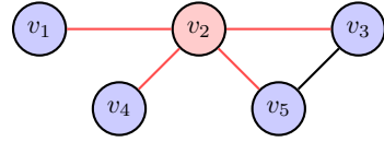
(a) Pick v_2 and encode its connections
