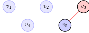
(b) Pick v_3 and encode its connections
