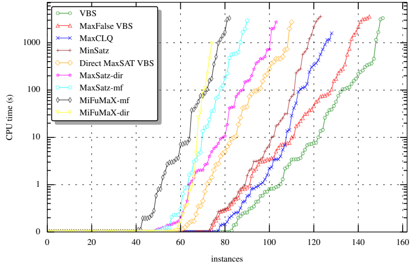
Fig. 6: Cactus plot showing the performance of the considered approaches
