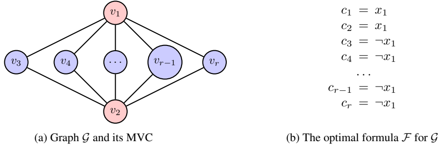
Fig. 5: Example of a graph \mathcal{G} , for which the size of the MVC of \mathcal{G} is greater than the minimum number of variables in the corresponding CNF formula \mathcal{F}
