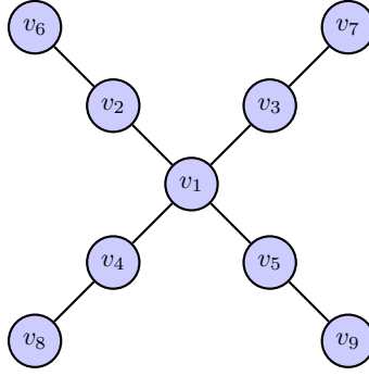
Fig. 3: Counterexample showing non-optimality of the greedy algorithm
