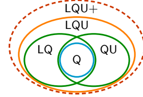
Fig. 2. Relations among the Proof Systems.
